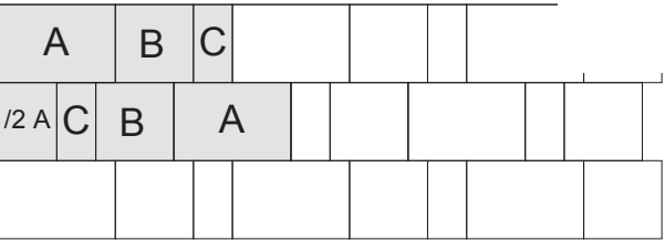
A - 63x42, B - 42x42, C- 21x42
